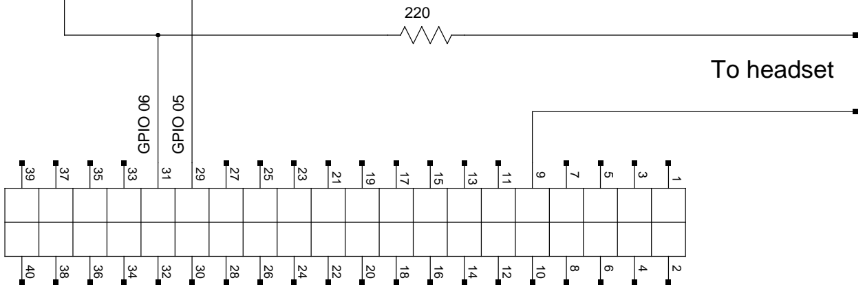
Raspberry Pi 2 Model B I/O Connector
